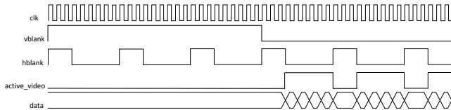
Fig. 2: Video timing signals
