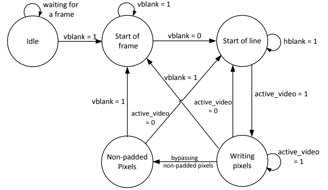
Fig. 5: The finite state machine for the writing process
