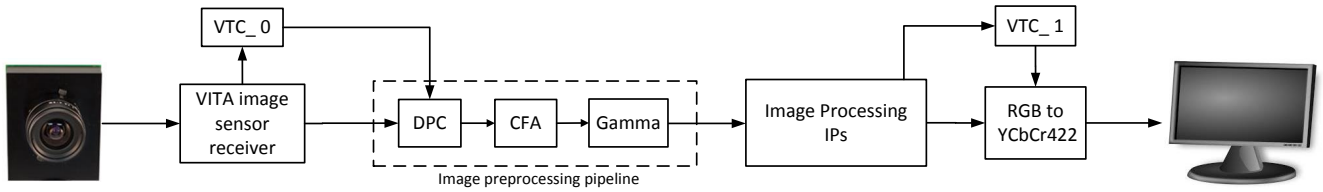
Fig. 1: Video processing system architecture
